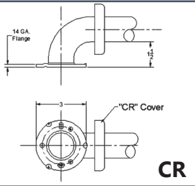
CONCEALED SCREW FLANGES
