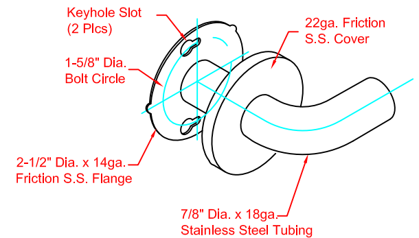
Mounting Flange Detail
